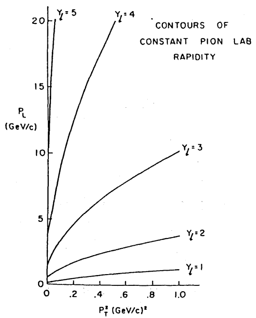
Fig. 12. Contours of constant pion lab rapidity.
