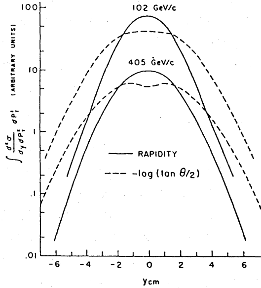
Fig. 11. Comparison between true rapidity and -\log(\tan \theta/2) .
